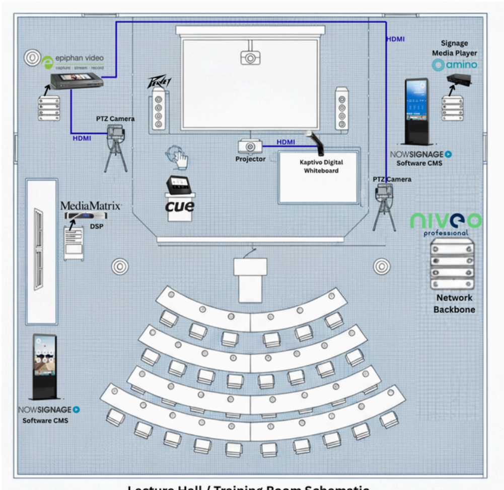
Lecture Hall / Training Room Schematic
