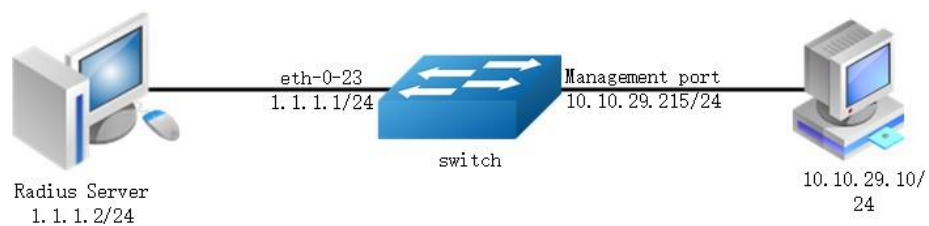
Figure 7-16 private vlan
