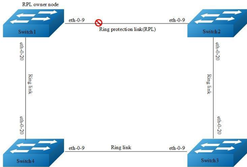
Figure 16-12 Topology of single G8032 ring
