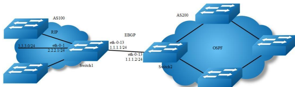
Figure 5-19 EBGP
