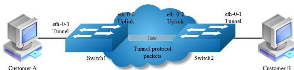
Figure 3-24 L2 protocol tunnel
