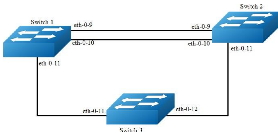
Figure 16-38 BFD single hop
