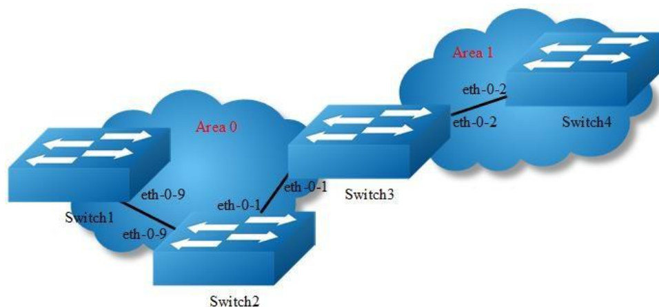
Figure 5-16 ospf authentication
