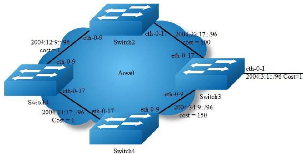
Figure 13-6 OSPFv3 Cost
