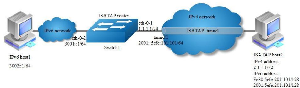
Figure 11-7 ISATAP tunnel
