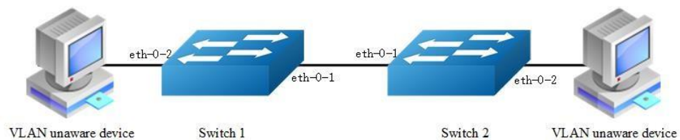
Figure 3-11 Trunk link
