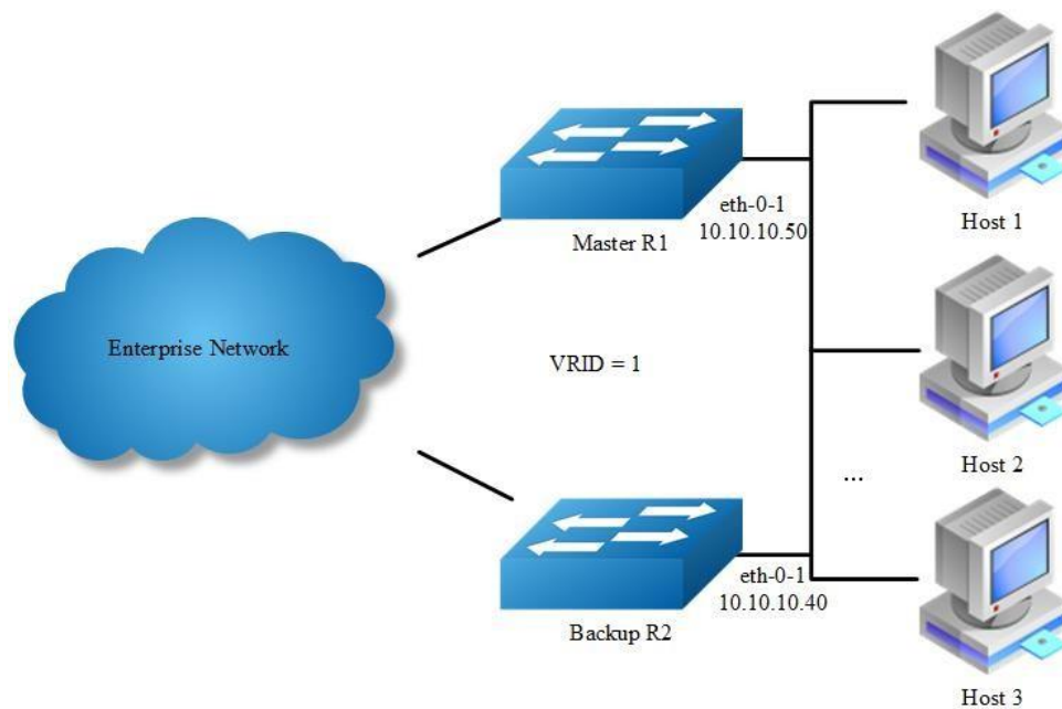
Figure 16-36 VRRP Track
