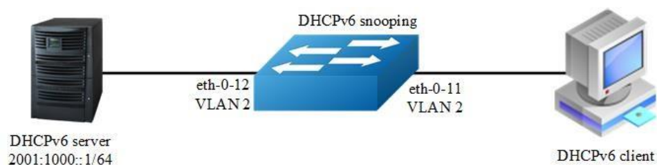
Figure 12-1 DHCPv6 Snooping
