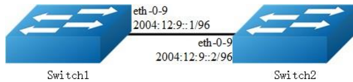
Figure 13-2 OSPFv3
