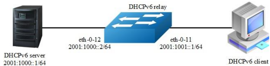
Figure 11-9 DHCP Relay
