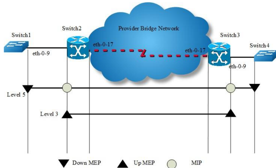
Figure 16-6 CFM
