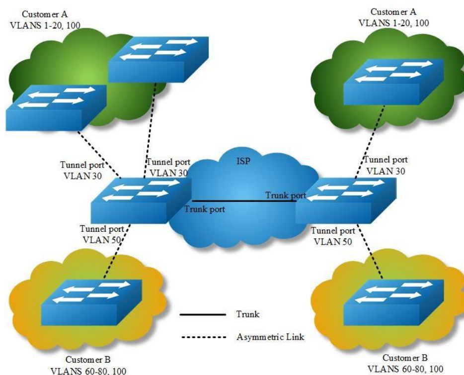
Figure 3-13 QinQ Tunnel
