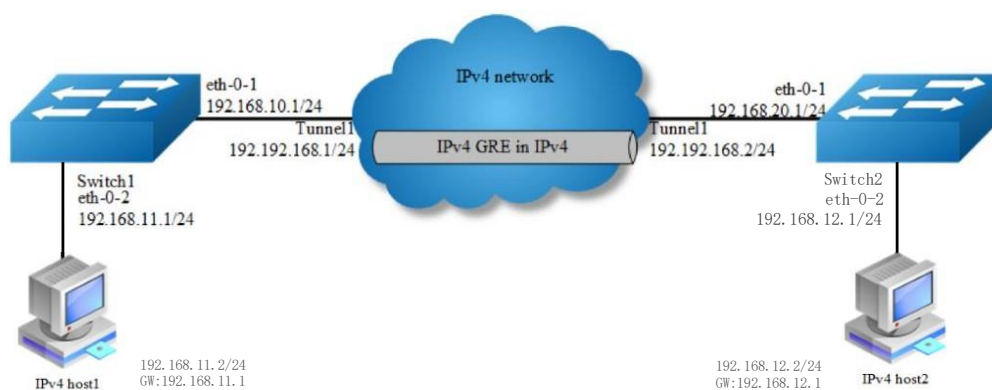
Figure 15-2 IPv4 gre Tunnel
