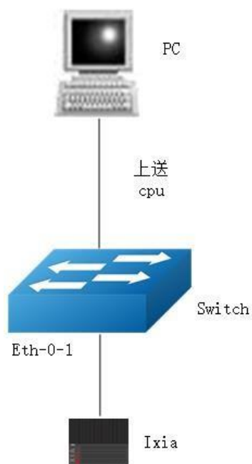
Figure 7-5 copp_acl
