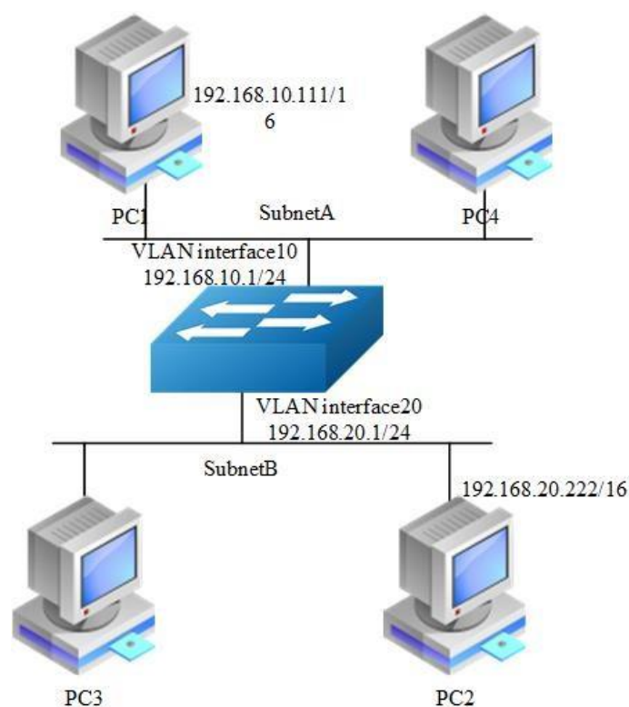
Figure 4-2 arp proxy
