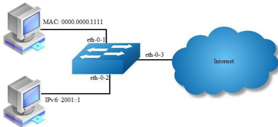
Figure 7-4 ipv6 acl
