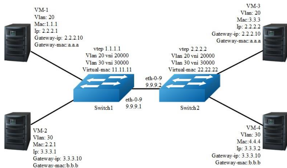
Figure 17-8 GENEVE
