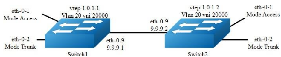
Figure 17-1 Vxlan
