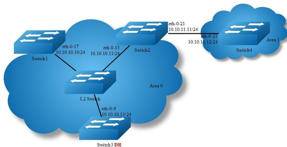
Figure 5-13 ospf area
