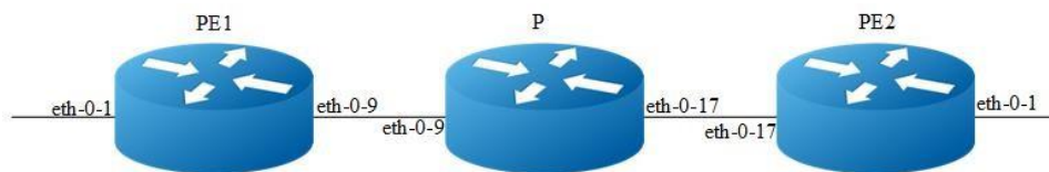
Figure 19-8 MPLS QoS LSP model
