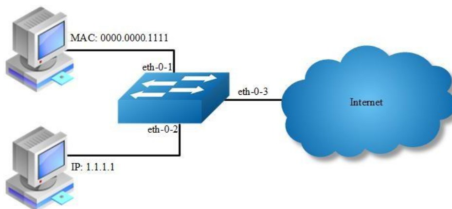
Figure 7-2 acl
