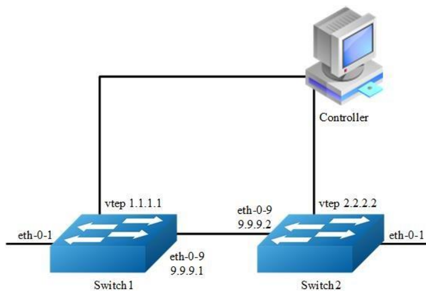
Figure 17-12 OVSDB
