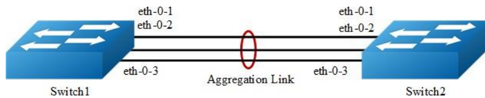
Figure 3-19 Static LACP
