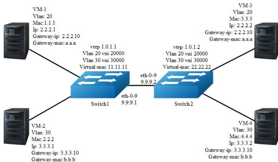
Figure 17-2 Vxlan
