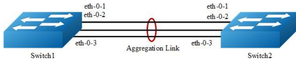
Figure 3-20 Static Agg
