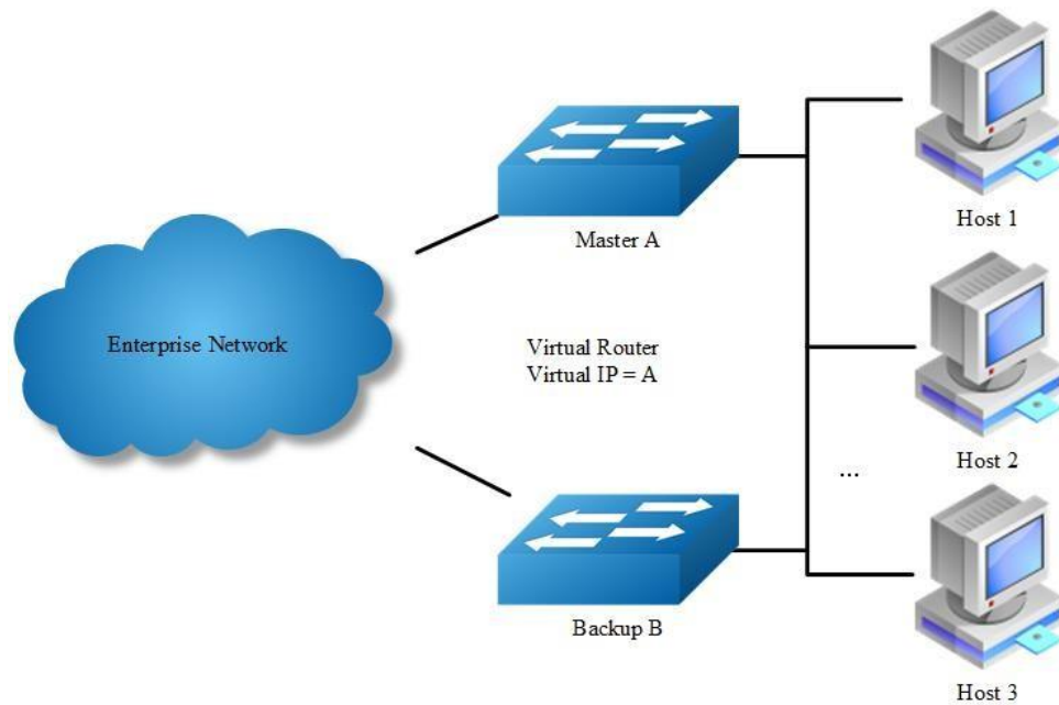
Figure 16-22 With VRRP
