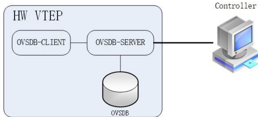
Figure 17-11 OVSDb
