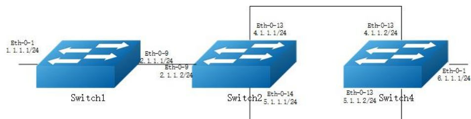
Figure 5-18 pbr
