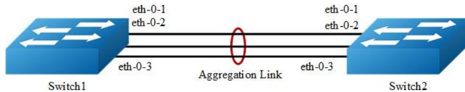
Figure 3-18 Dynamic LACP
