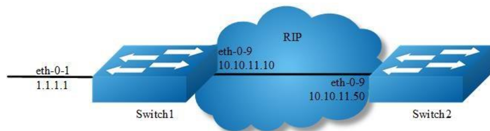
Figure 5-7 rip split-horizon
