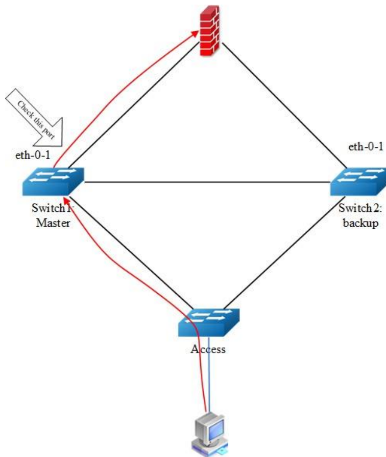
Figure 16-32 Track interface
