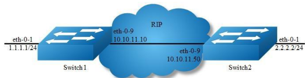
Figure 5-9 rip authentication
