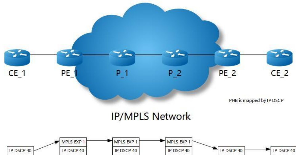
Figure 19-7 Short pipe model
