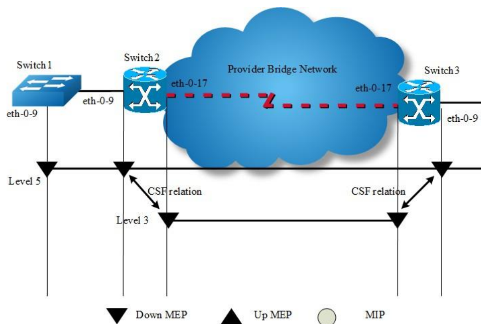
Figure 16-7 CFM CSF
