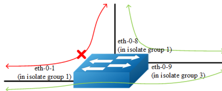
Figure 7-27 Port Isolate
