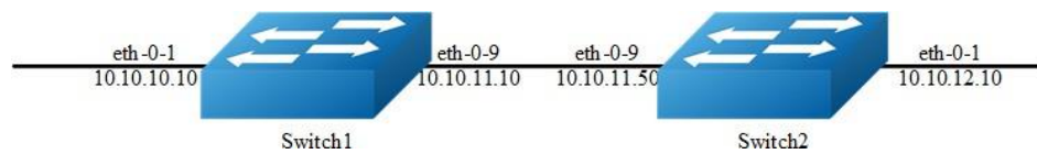
Figure 5-2 enable rip
