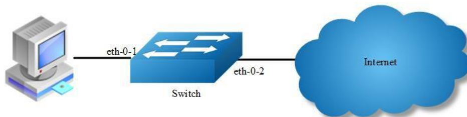
Figure 7-3 extern acl
