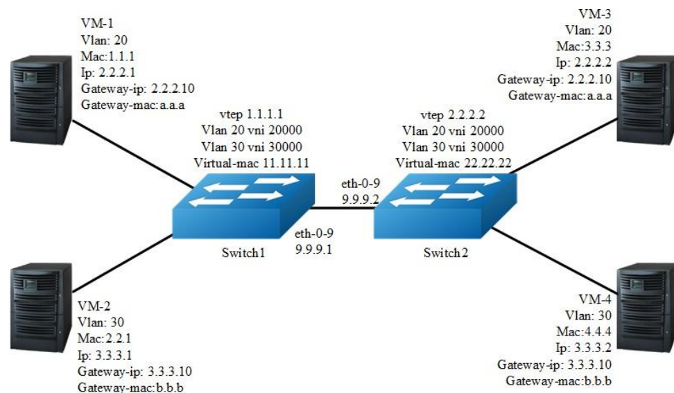
Figure 17-6 NVGRE
