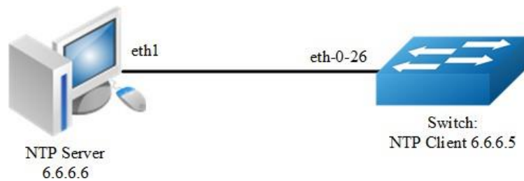
Figure 9-1 NTP
