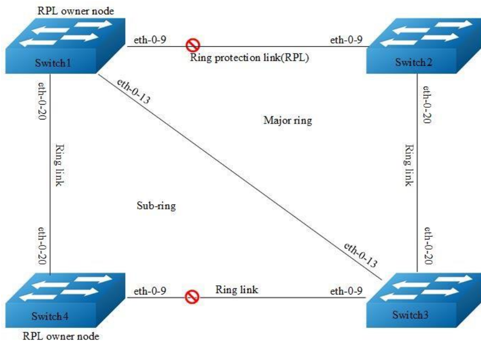
Figure 16-13 Topology of multiple G8032 rings
