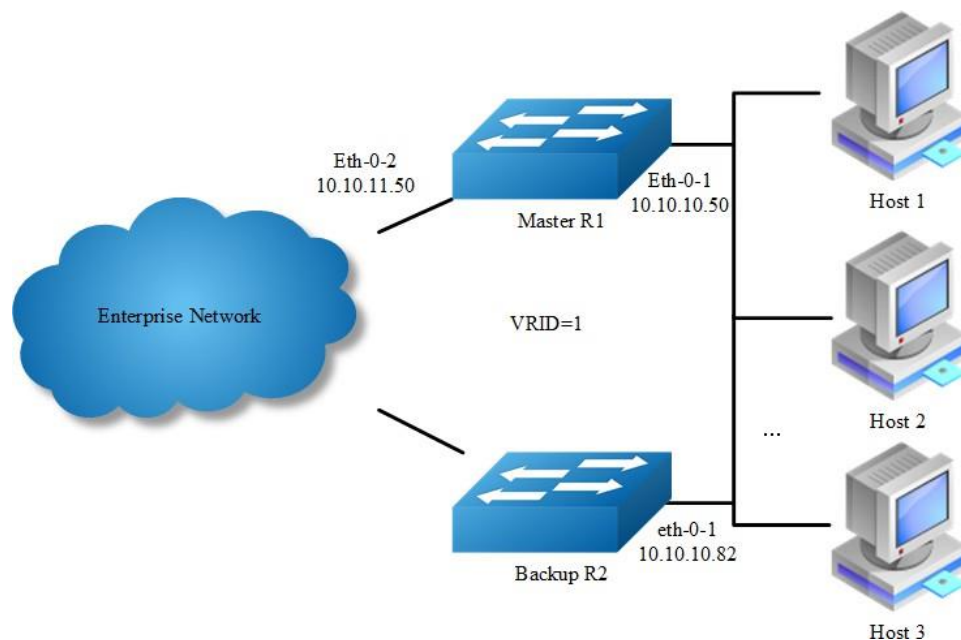
Figure 16-25 VRRP Circuit Failover
