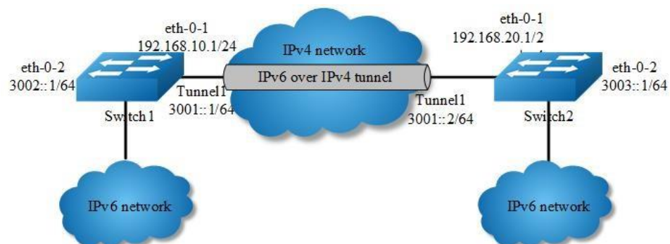
Figure 11-4 Manual Tunnel
