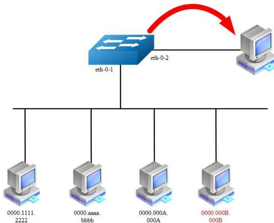
Figure 7-1 Port Security
