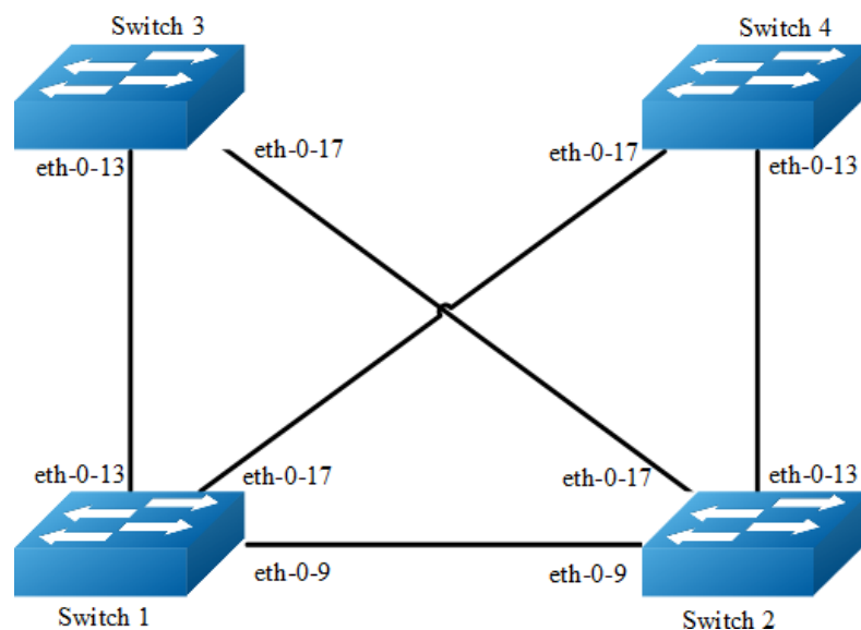
Figure 16-19 Multilink-enhance Typical Topology
