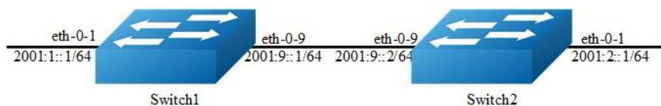
Figure 14-1 PIMv6 Sparse-mode
