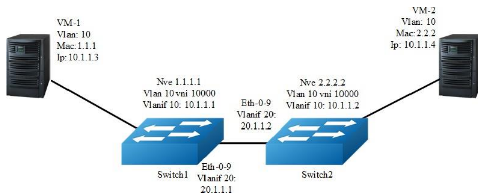
Figure 17-3 EBGp_EVPN
