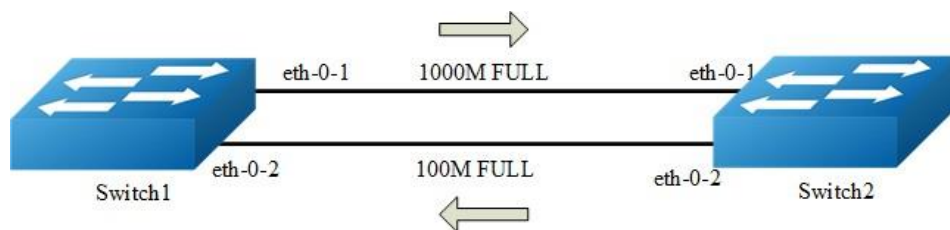
Figure 3-21 Flow control
