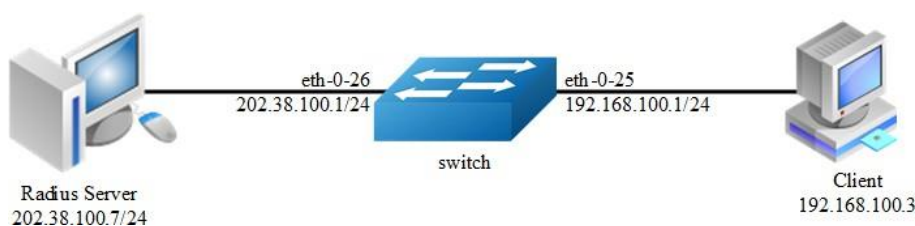
Figure 7-6 dot1x
