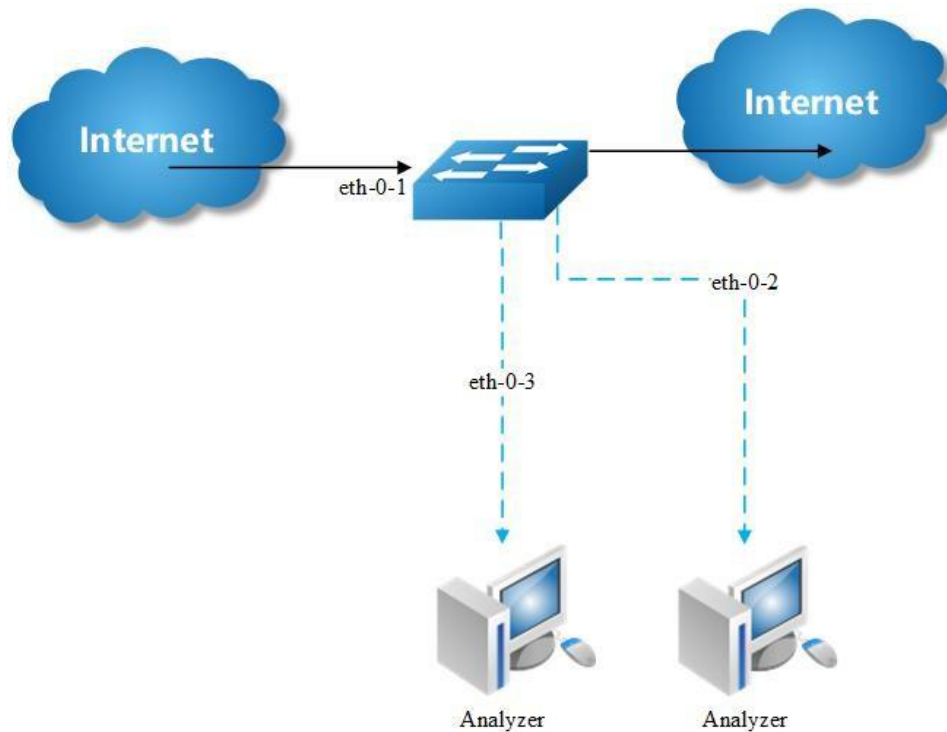
Figure 8-5 Multi-destination Mirror
