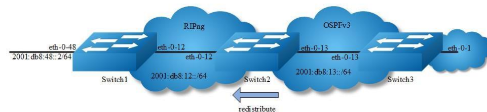
Figure 13-10 RIPng redistribute
