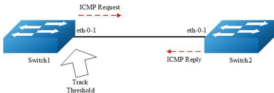
Figure 16-34 Track ip sla
