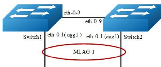
Figure 3-26 MLAG
