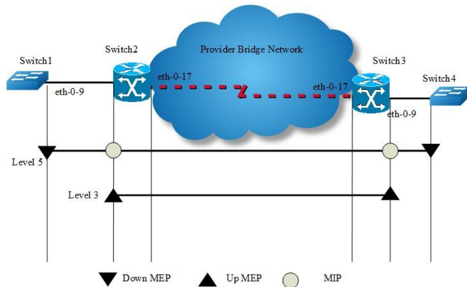
Figure 16-9 CFM
