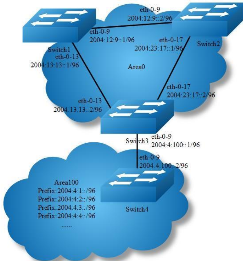
Figure 13-4 OSPFv3 area
