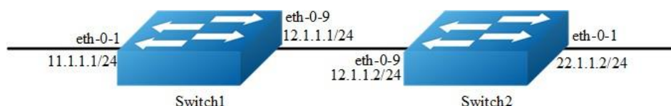
Figure 6-1 Pim sm
