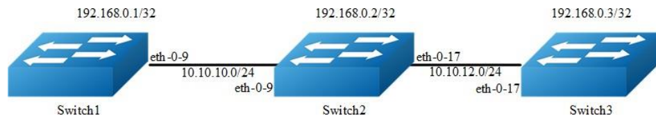
Figure 5-1 ip unicast routing
