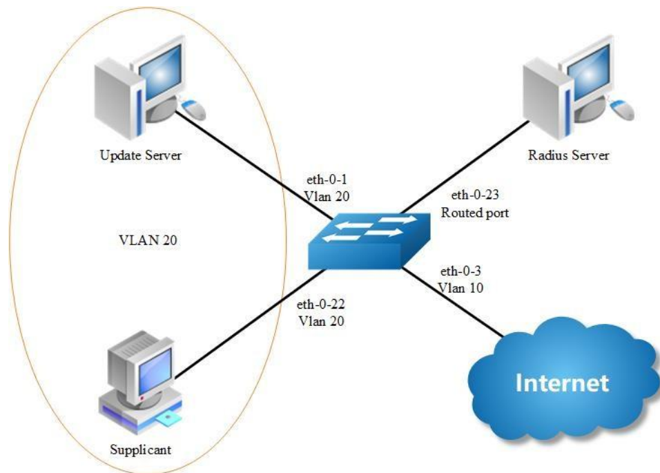
Figure 7-10 Guest vlan: before authenticated
