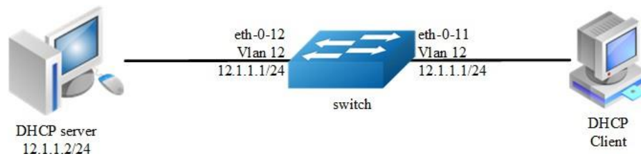
Figure 7-13 dhcp snooping
