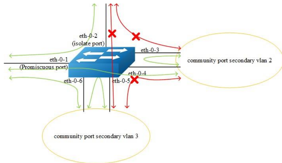
Figure 7-15 private vlan
