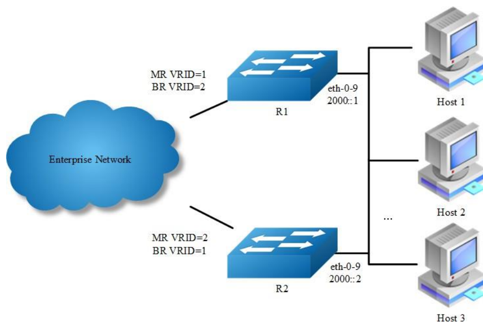
Figure 16-27 IPv6 VRRP with two virtual router
