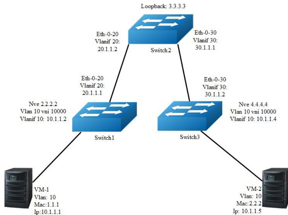
Figure 17-4 IBGP_EVPN
