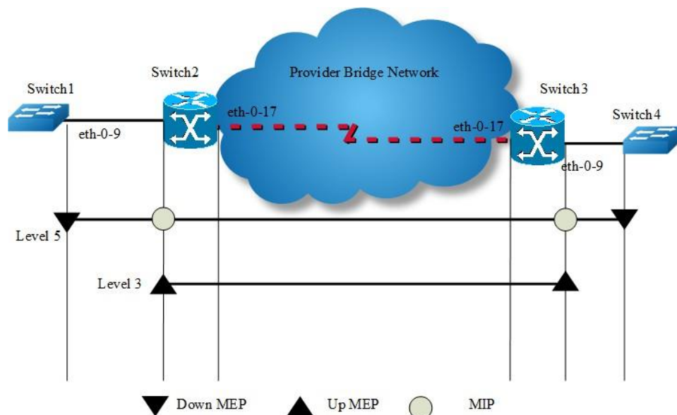
Figure 16-8 CFM
