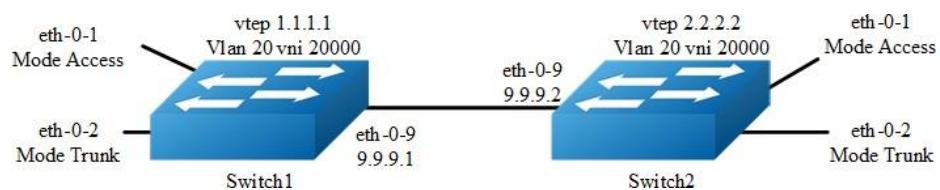
Figure 17-7 GENEVE
