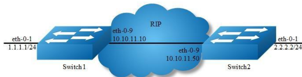
Figure 5-10 rip authentication
