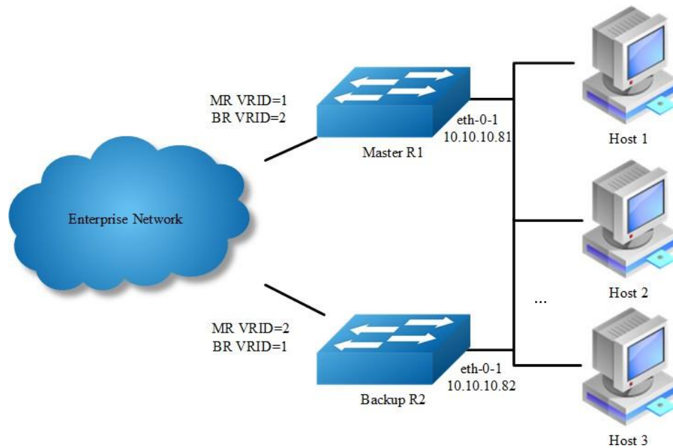
Figure 16-24 VRRP with two virtual router
