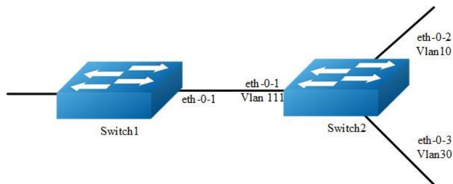
Figure 6-4 mvr
