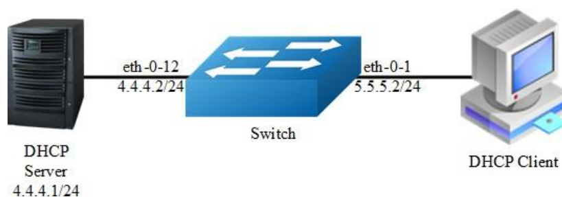
Figure 4-5 DHCP relay
