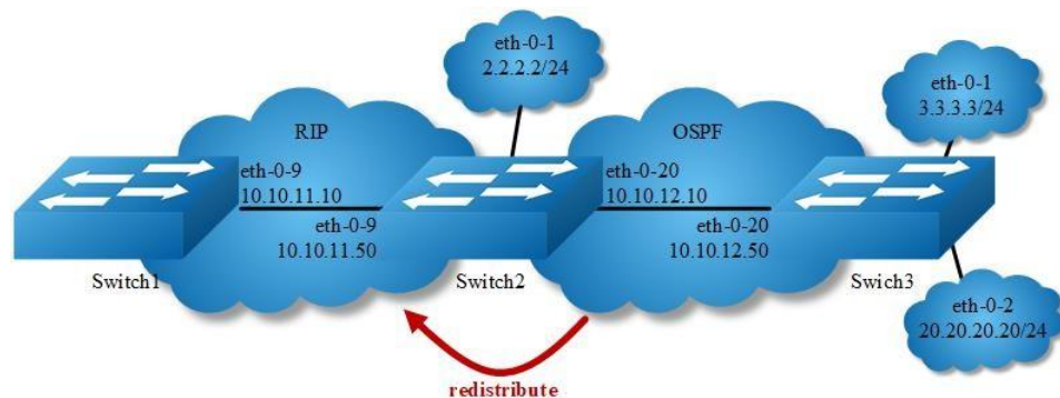
Figure 5-6 rip redistribute
