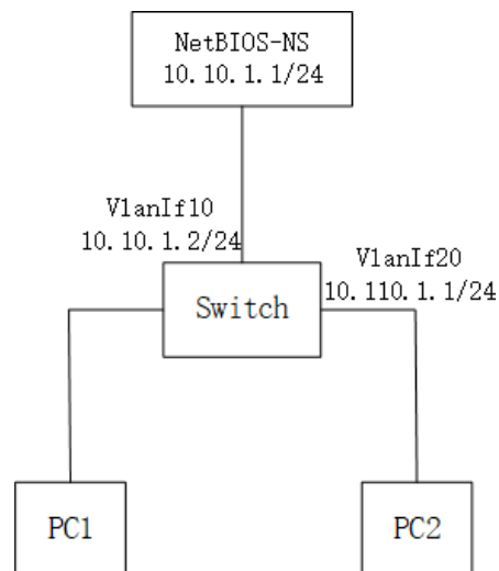
Figure 16-41 UDP-Helper configuration
