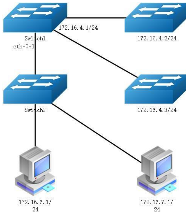
Figure 5-17 pbr
