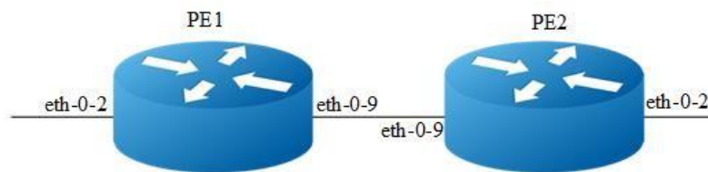
Figure 19-4 Topology of vpws configuration
