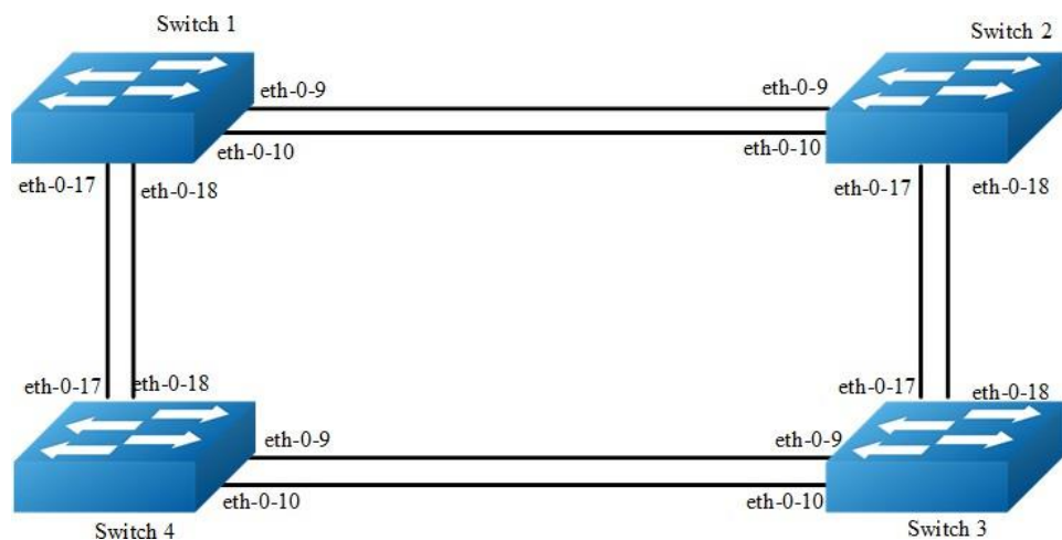
Figure 3-25 MSTP
