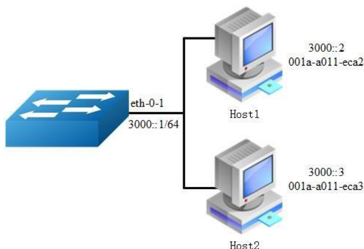
Figure 11-8 NDP
