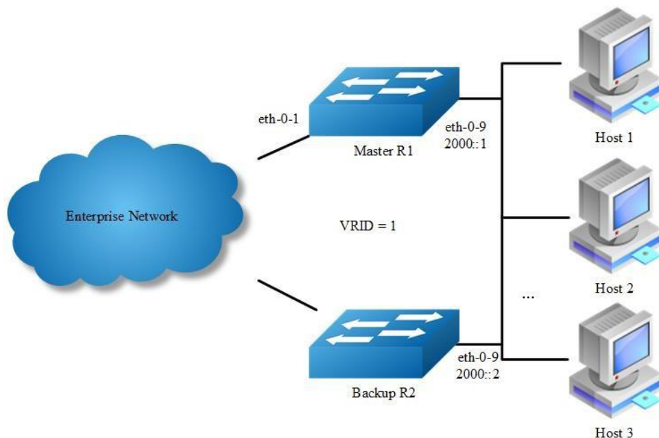
Figure 16-28 IPv6 VRRP Circuit Failover
