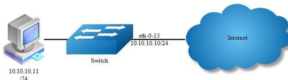
Figure 7-28 Topology for DDoS test
