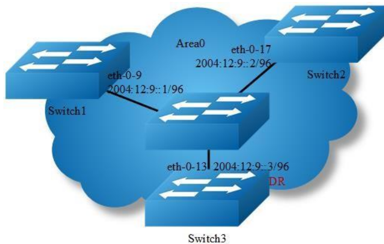
Figure 13-3 OSPFv3 priority
