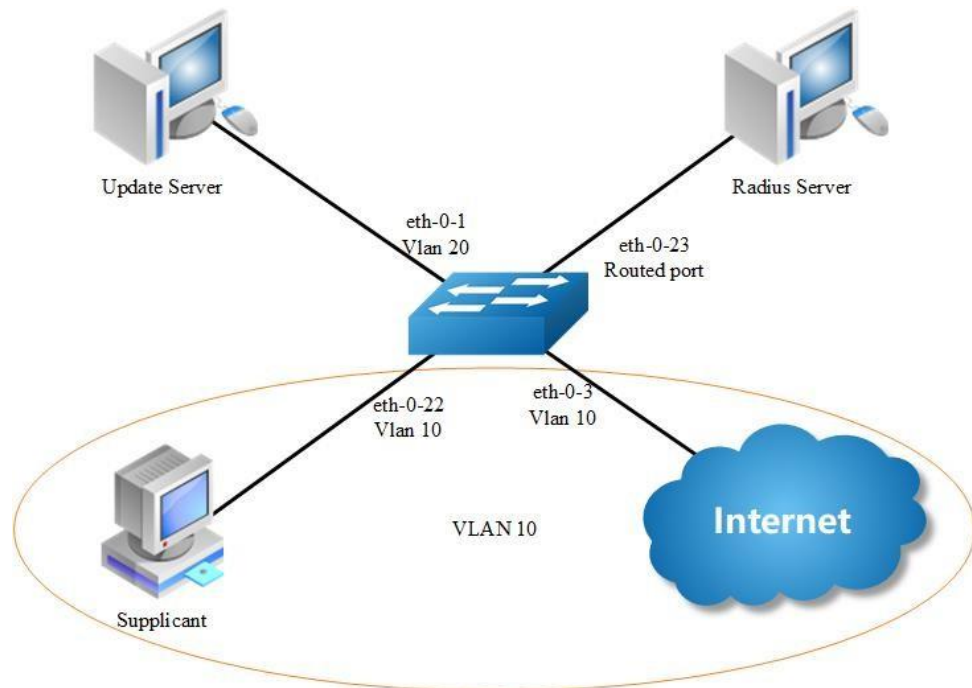
Figure 7-11 Guest vlan: after authenticated
