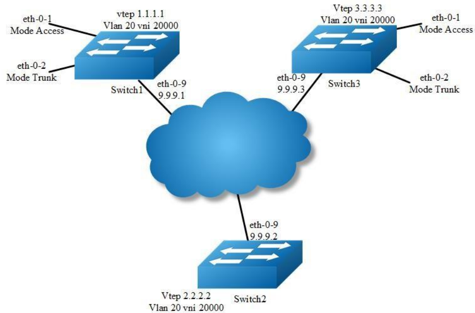
Figure 17-10 OVERLAY without Horizon Split
