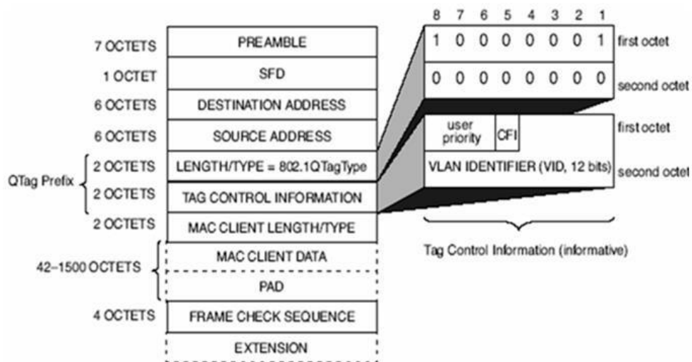
Figure 3-7 Tagged Frame
