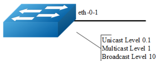
Figure 3-22 Percentage Storm Control
