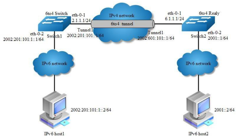
Figure 11-6 6to4 relay
