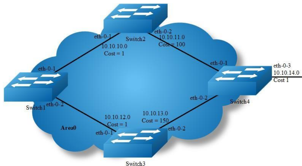
Figure 5-15 ospf cost
