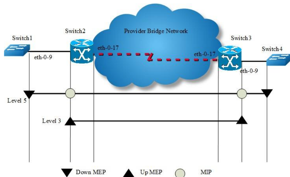
Figure 16-10 CFM
