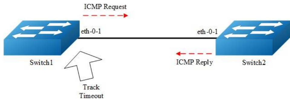
Figure 16-33 Track ip sla
