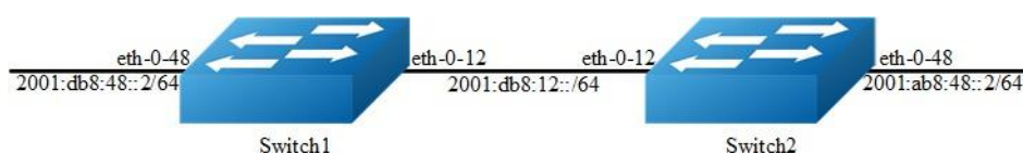
Figure 13-7 RIPng
