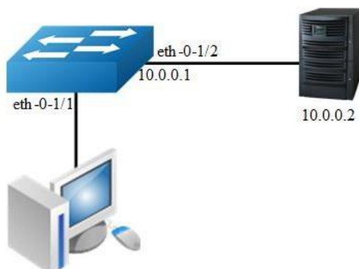
Figure 18-2 EFD
