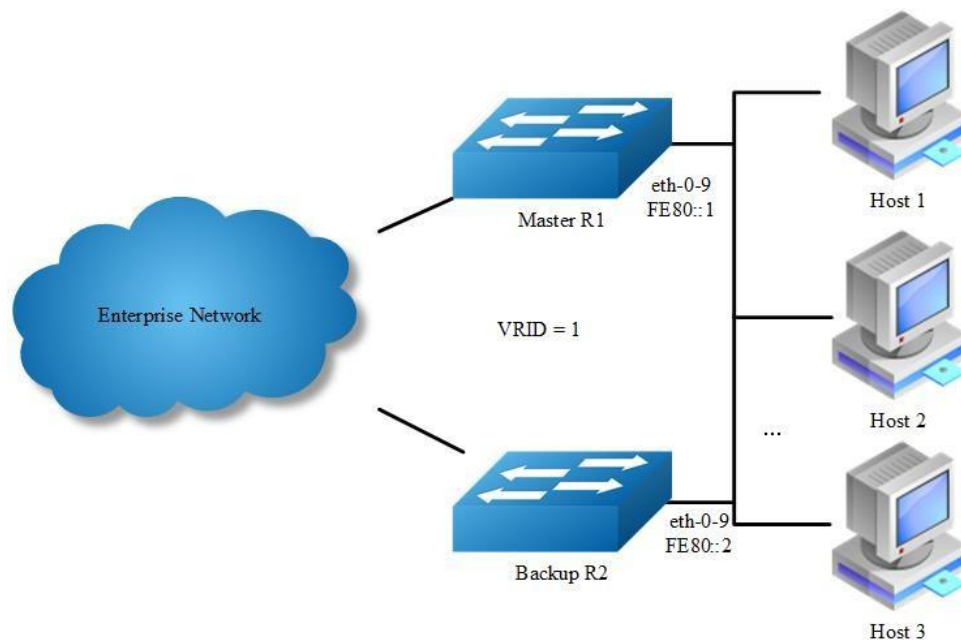
Figure 16-26 IPv6 VRRP with one virtual router
