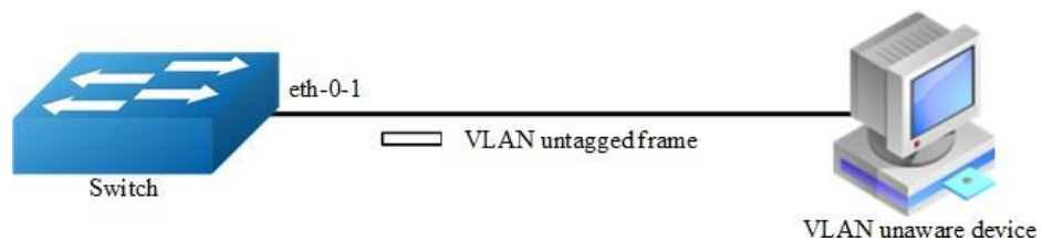
Figure 3-10 Access link
