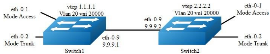
Figure 17-5 NVGRE
