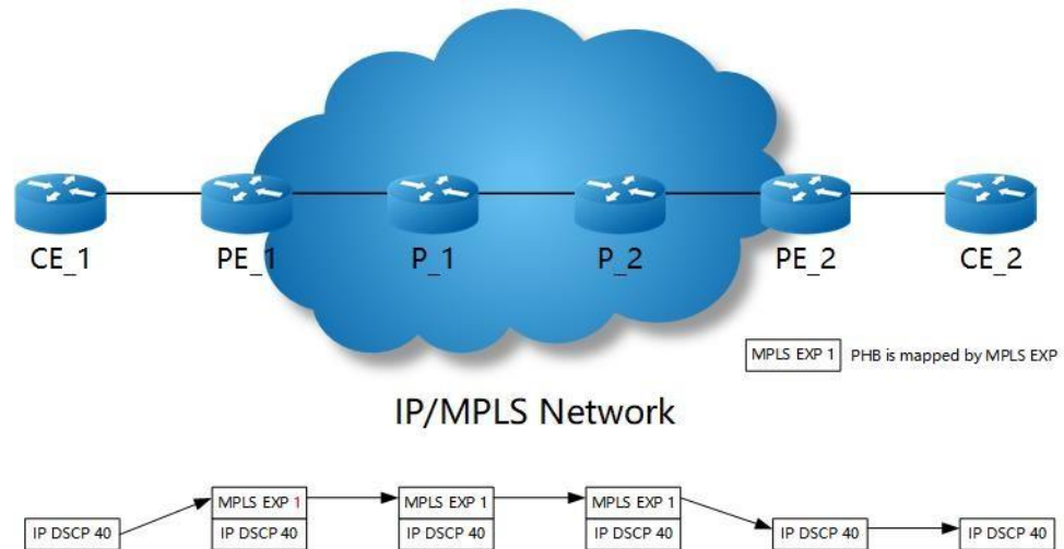
Figure 19-6 Pipe model
