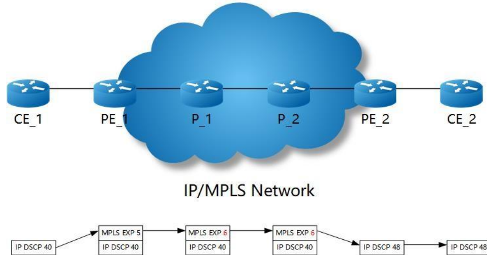
Figure 19-5 Uniform model
