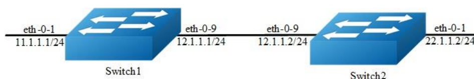
Figure 6-3 Pim dm
