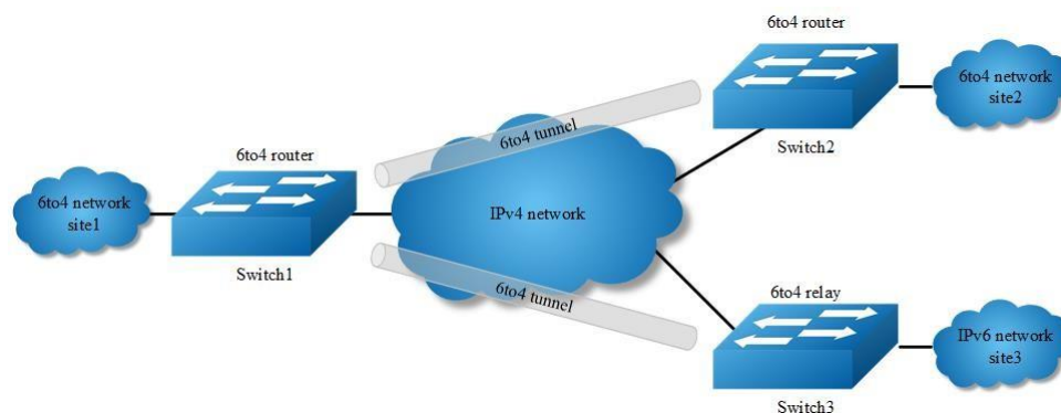
Figure 11-2 IPv6 over IPv4 Tunnel
