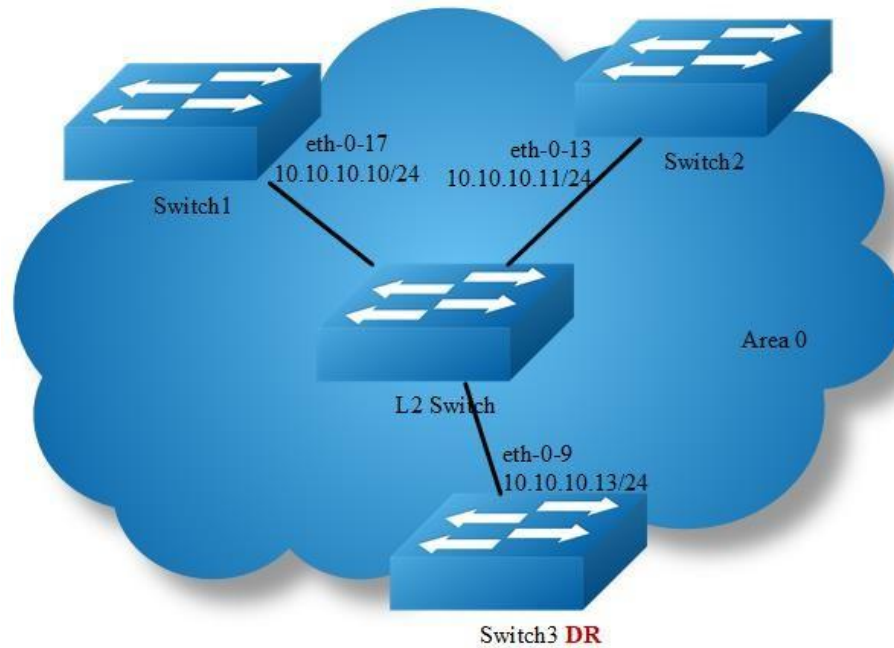
Figure 5-12 ospf priority
