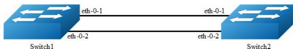
Figure 6-2 bsr
