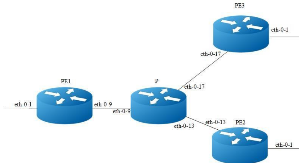
Figure 19-3 VPLS model
