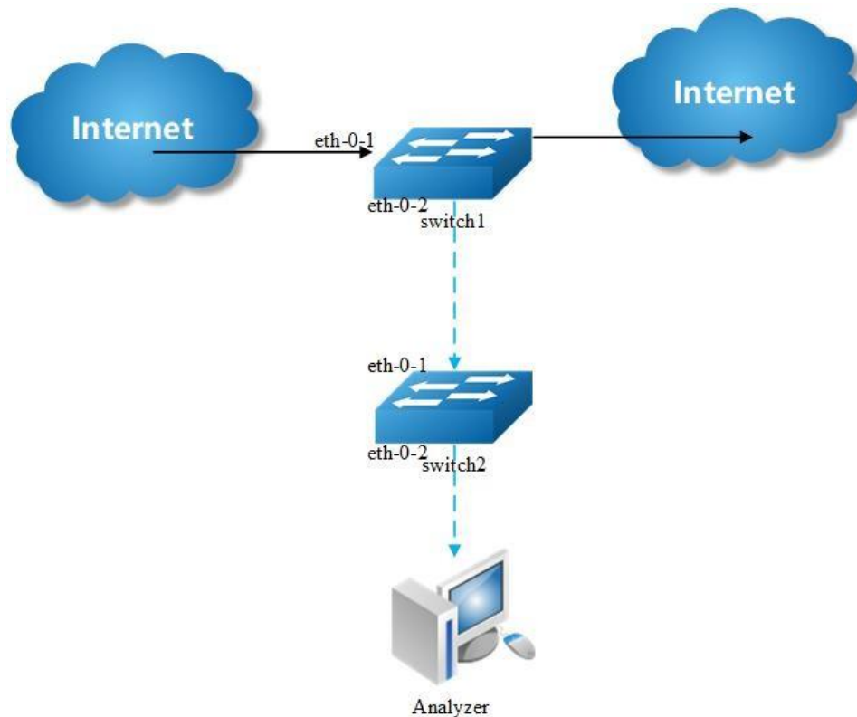
Figure 8-6 Remote Mirror
