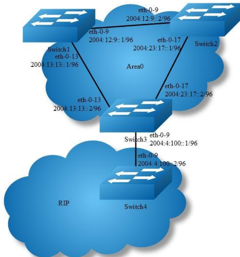
Figure 13-5 OSPFv3 Redistribute
