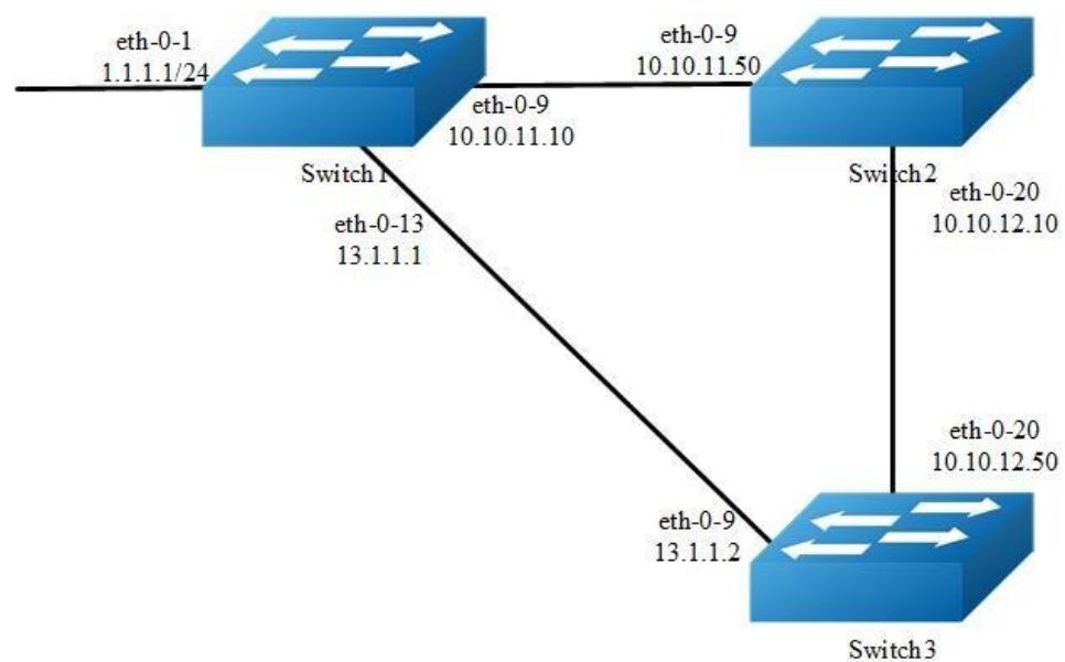
Figure 5-4 rip metric
