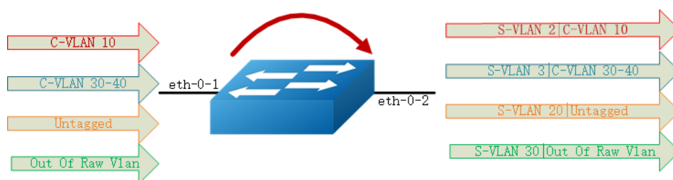
Figure 3-16 QinQ Tunnel
