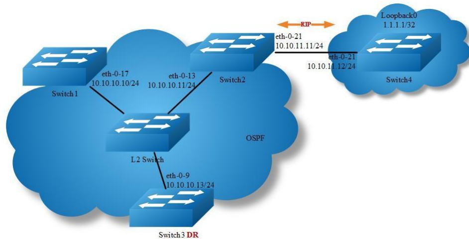
Figure 5-14 ospf redistribute
