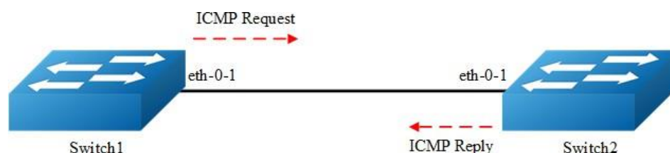
Figure 16-29 IP SLA
