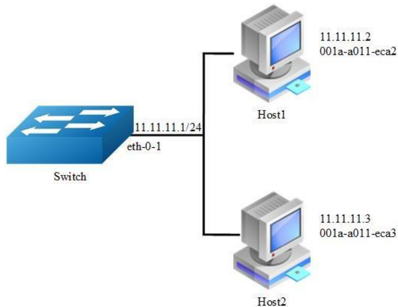
Figure 4-1 arp
