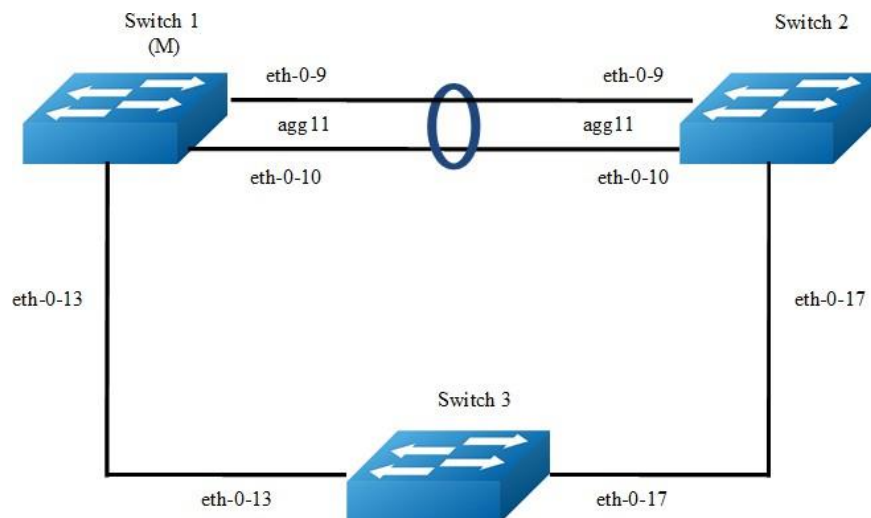
Figure 16-15 ERPS
