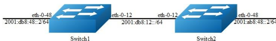
Figure 13-11 RIPng Split-horizon
