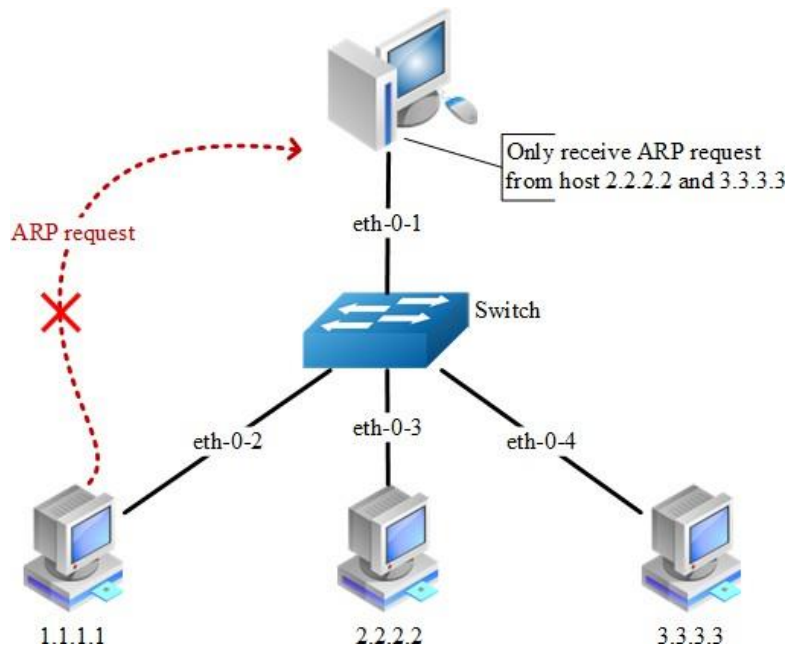
Figure 7-12 arp inspection
