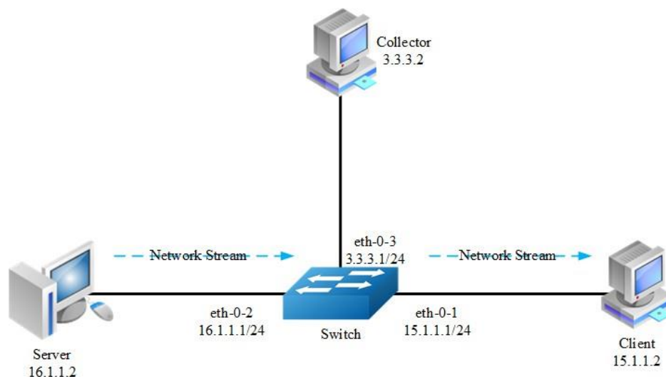
Figure 9-8 sflow
