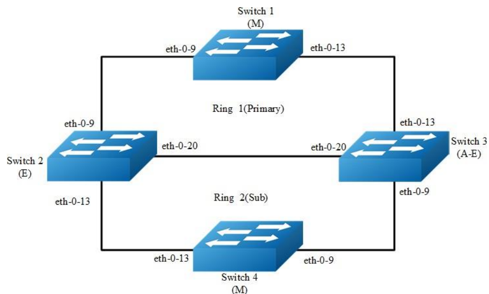
Figure 16-16 ERPS
