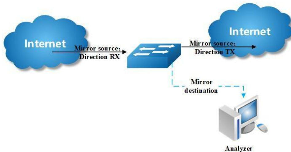
Figure 8-3 Mirror
